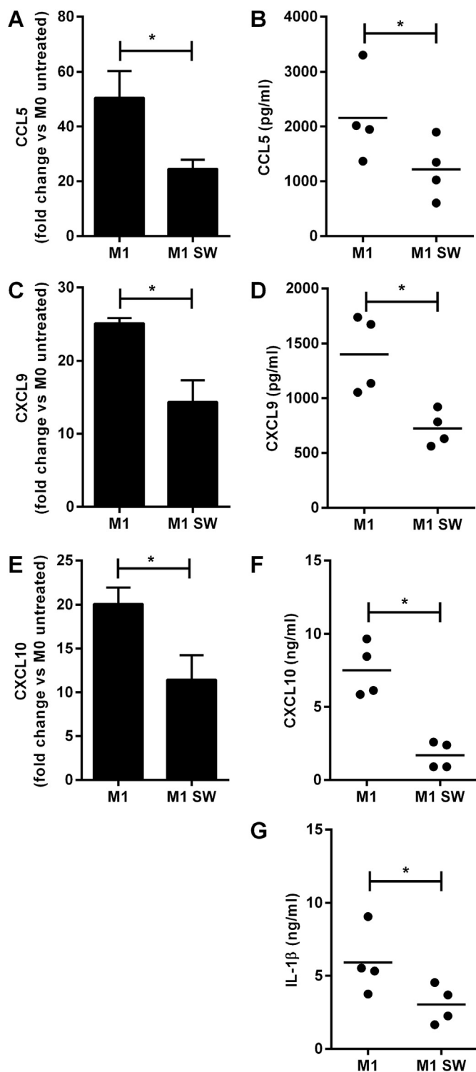
Fig. 3. SW inhibits expression and secretion of pro-inflammatory cytokines by M1 macrophages. Macrophages were stimulated with LPS plus IFN- \gamma for 24 h (M1) and subsequently exposed or not to 322 mJ SW (M1 SW). After 4 h, gene transcript levels and cytokine concentrations in cell-free supernatants were measured for CCL5 (A and B), CXCL9 (C and D), CXCL10 (E and F), and IL-1 \beta (G). Results are expressed as mean \pm SEM of 4 independent experiments. * p < 0.05 by t-test.
