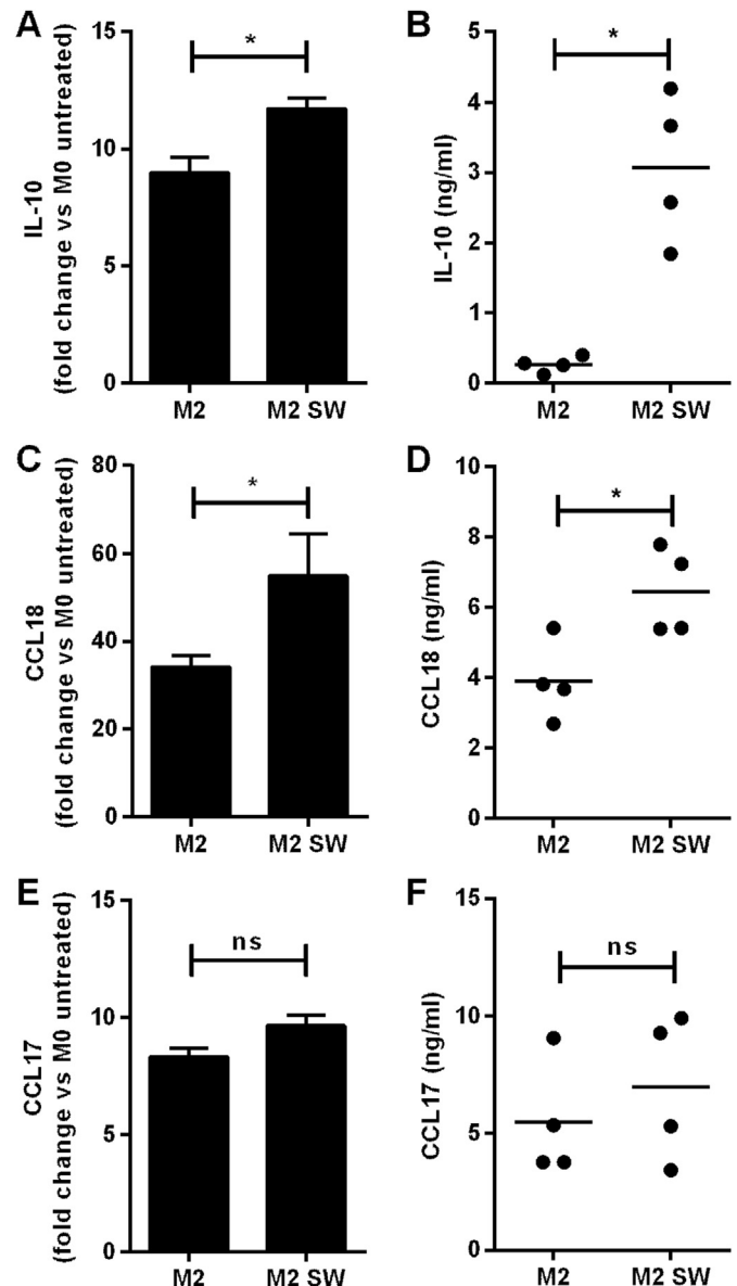
Fig. 5. SW effects on M2-related cytokines in alternative activated macrophages. Macrophages were stimulated with IL-4 for 24 h (M2) and subsequently exposed or not to 322 mJ SW (M2 SW). After 4 h, gene transcript levels and cytokine concentrations in cell-free supernatants were measured for IL-10 (A and B), CCL18 (C and D), and CCL17 (E and F). Results are expressed as mean \pm SEM of 4 independent experiments. * p < 0.05 by t-test.
